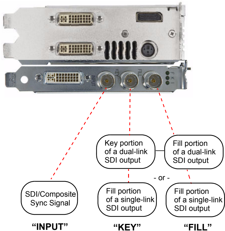
Figure 2.4 NVIDIA Quadro FX SDI Connectors
