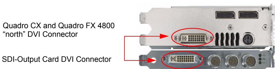
Figure 2.1 DVI Connection between the SDI Output card and the Quadro CX/QuadroFX 4800
