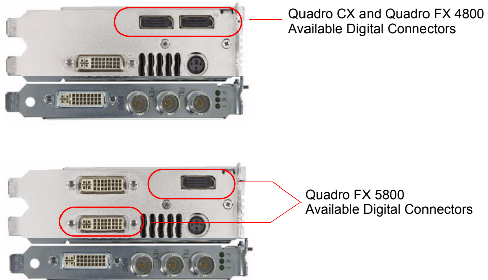
Figure 2.3 Digital Connectors Available for Displays
