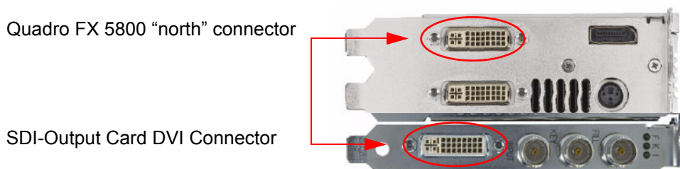
Figure 2.2 DVI Connection between the SDI Output card and the Quadro FX 5800
